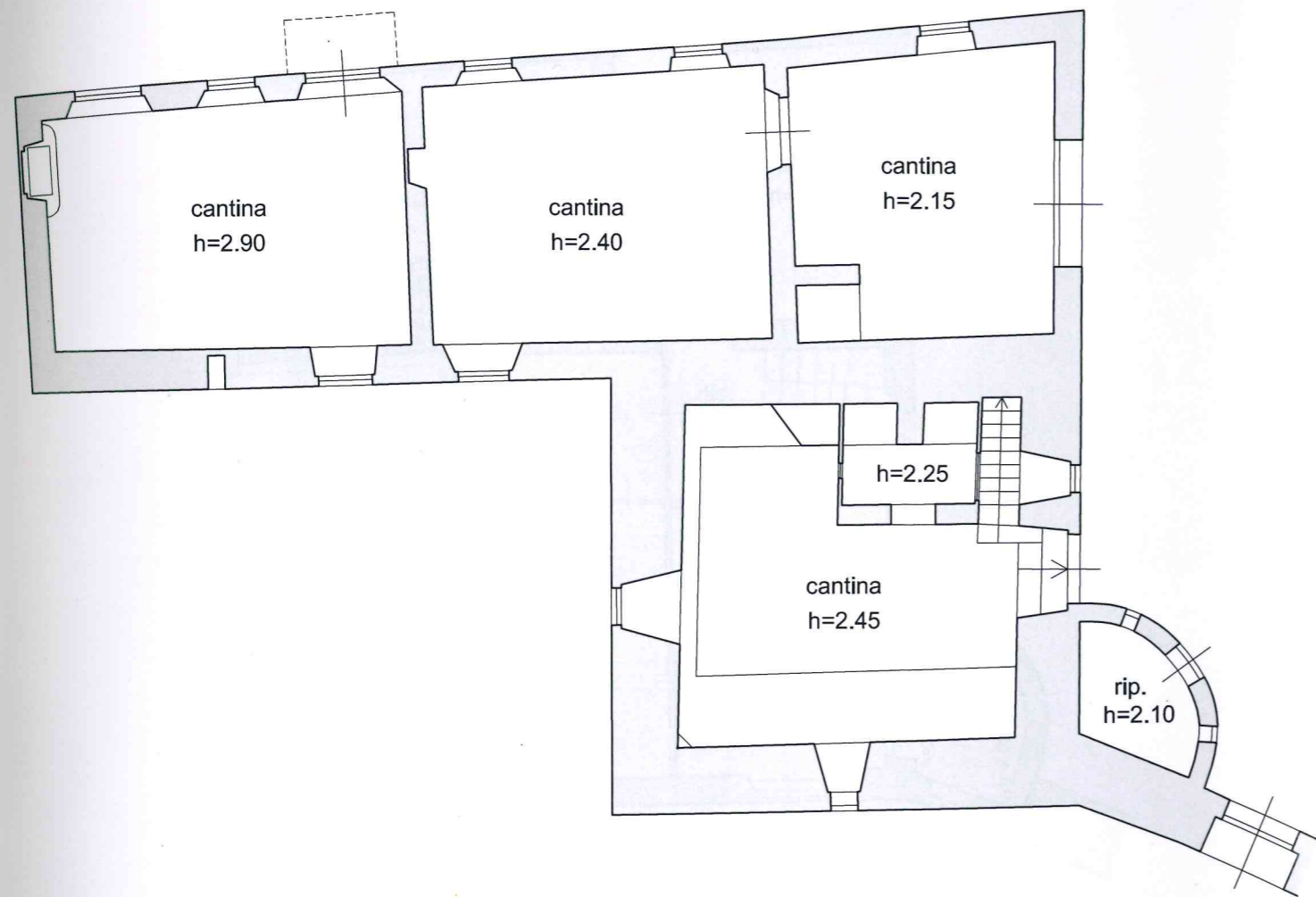
PIANO SEMINTERRATO
